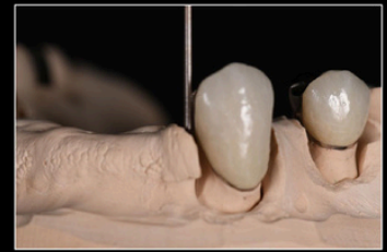
Milled Occlusal Rest and Guide Plane
